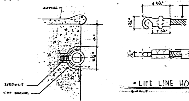
EYEBOLT AND CUP ANCHOR DETAIL SCALE 3/8" = 1'-0"
