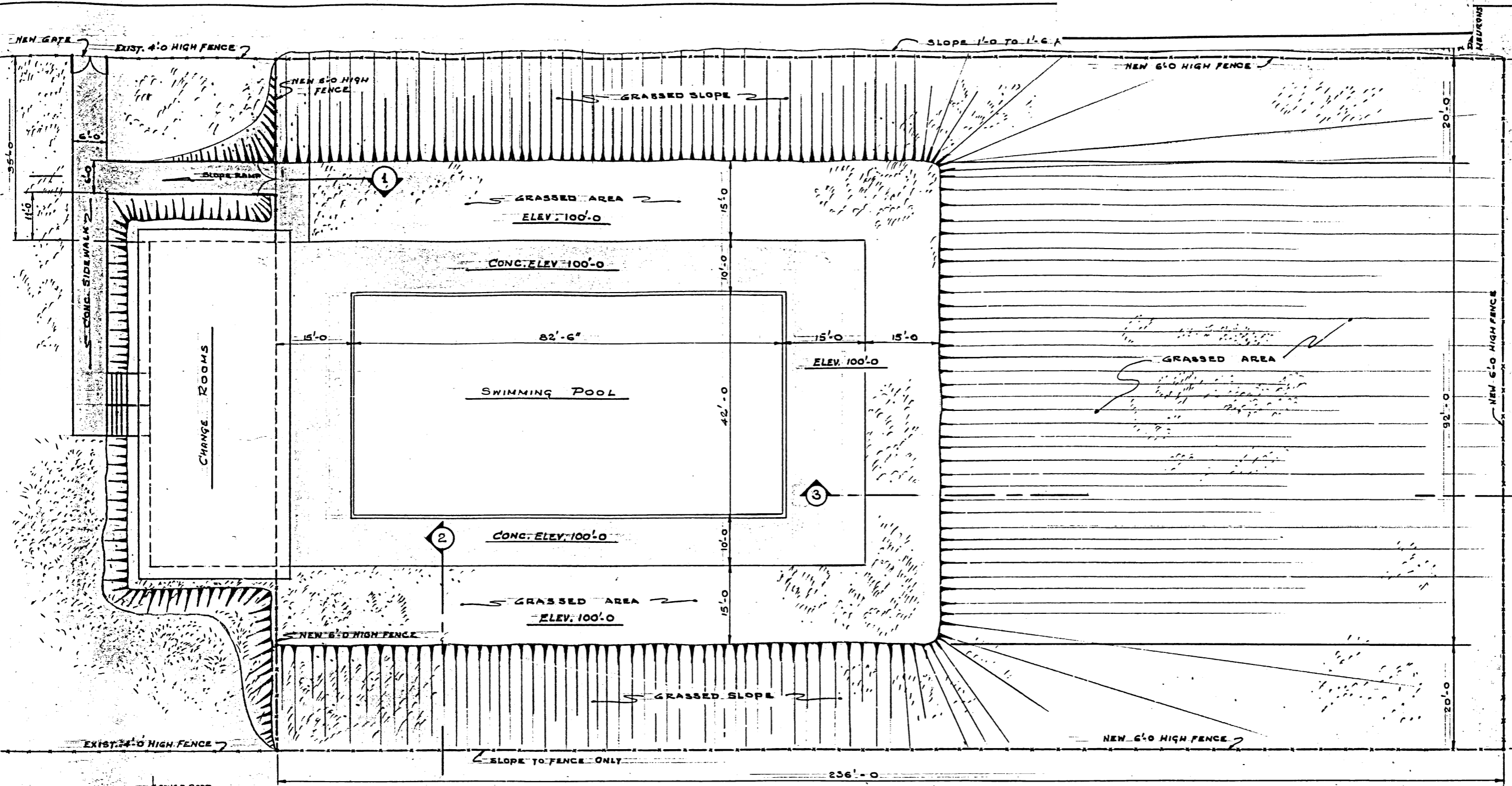
POOL AREA GRADING PLAN SCALE: 1" = 10'
