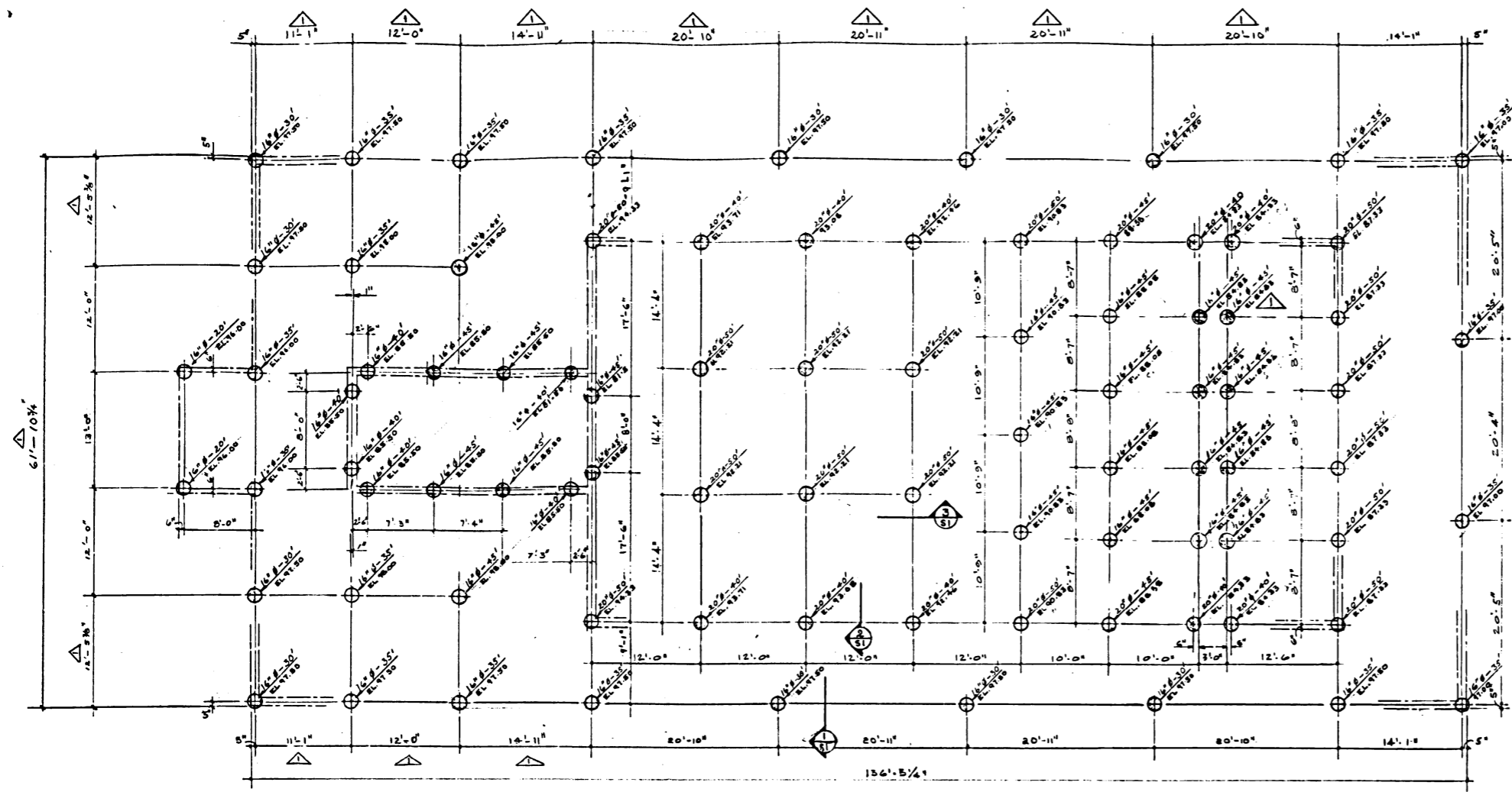
PILE LAYOUT 1/8" = 1'-0"
